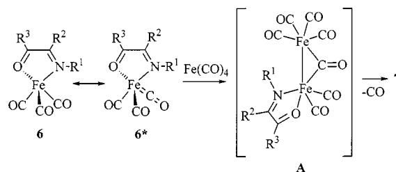
Scheme 4. Proposed reaction mechanism for the formation of 7
