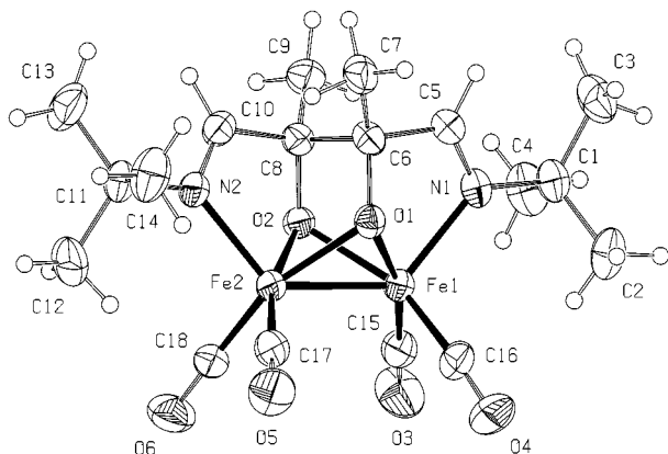
Figure 3. ORTEP drawing (50% probability level) of the molecular structure of 8a
