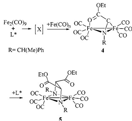
Scheme 2. Reaction of [Fe 2 (CO) 9 ] with PhCH(Me)N=C(H)–C(OEt)=O (L*)
