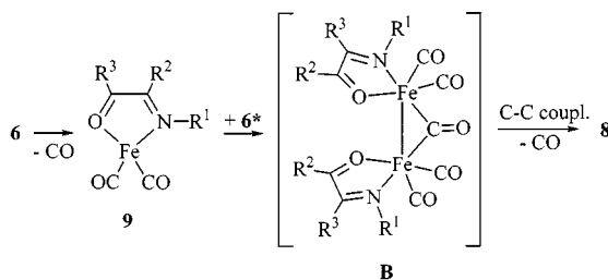
Scheme 5. Proposed reaction mechanism for the formation of 8
