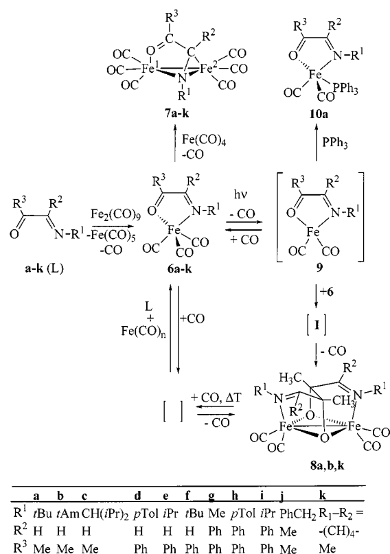
Scheme 3. Observed reaction sequence for [Fe 2 (CO) 9 ] with the \alpha -imino ketones a–k
