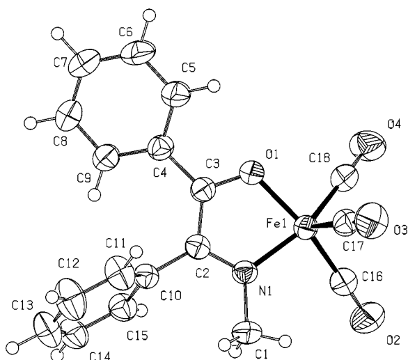
Figure 1. ORTEP drawing (50% probability level) of the molecular structure of 6g
