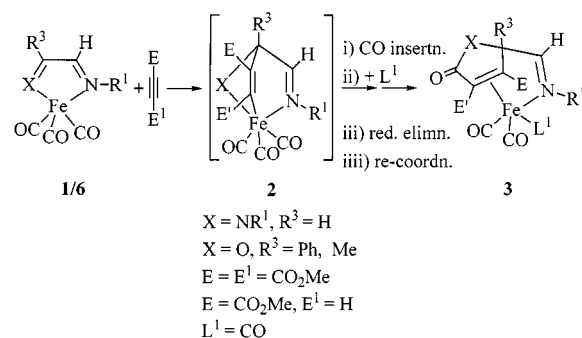
Scheme 1. Reactions of [\text{Fe}(\text{CO})_3\{\text{R}^1\text{N}=\text{C}(\text{H})-(\text{R}^3)\text{C}=\text{X}\}] ( \text{X} = \text{NR}^1, \text{O} ) with electron-deficient alkynes
