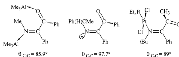
Figure 2. Torsion angles around the central \text{C}-\text{C} bond of coordinated and free \alpha -imino ketones
