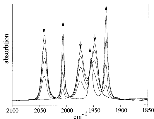
Figure 4. IR-spectral changes in the terminal carbonyl region during the irradiation of [\text{Fe}(\text{CO})_3\{t\text{BuN}=\text{C}(\text{H})-\text{C}(\text{Me})=\text{O}\}] ( 6a ) in toluene at 293 K (514.5 nm); formation of 8a
